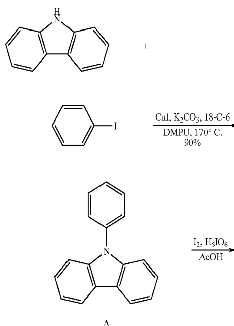
Reaction Scheme 2
