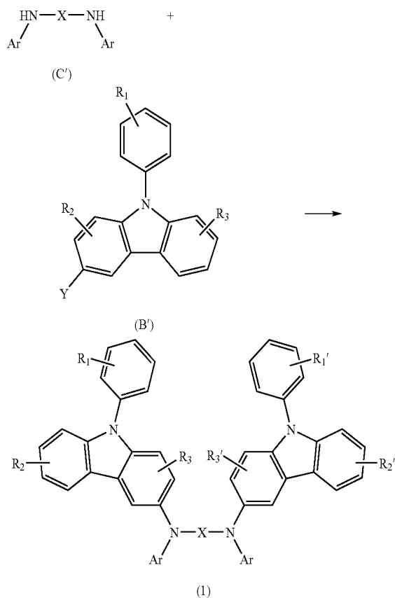
Reaction Scheme 1
